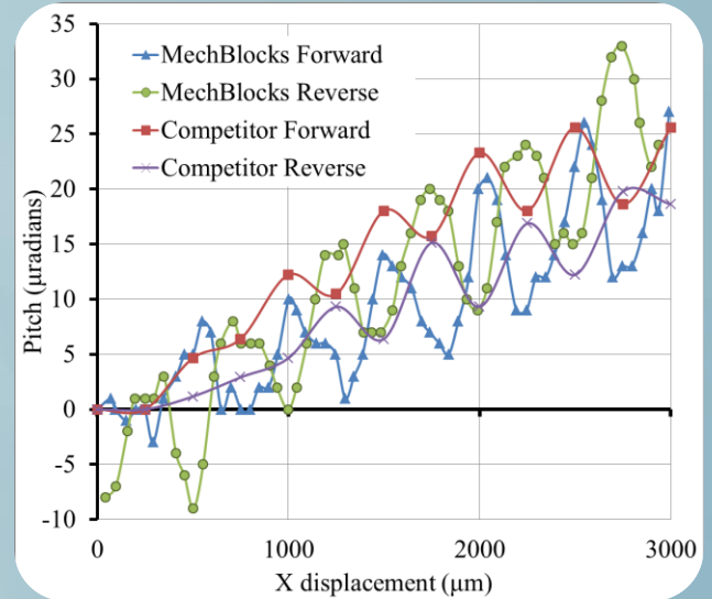
MechBlocks double-compound linear flexure translator comparison.
